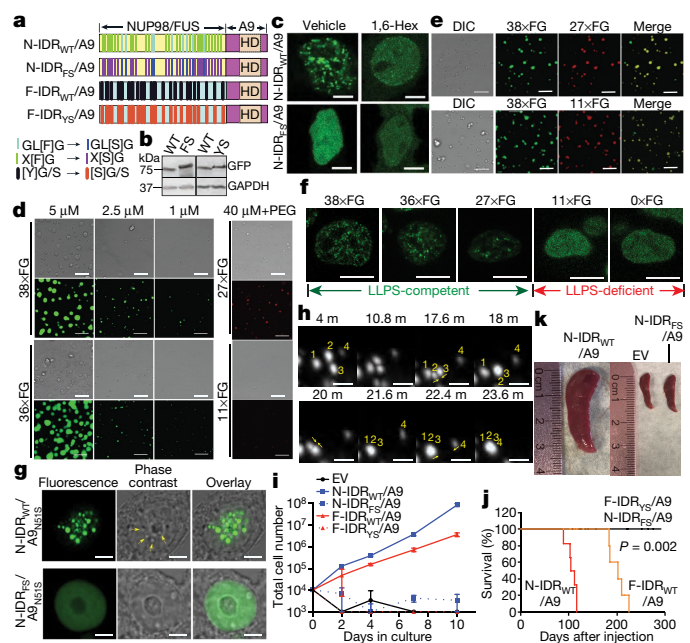
Fig. 1 | IDRs within chimeric transcription factor oncroteins establish phase-separated assemblies, inducing leukaemogenesis. a , Scheme for N-IDR/A9 and F-IDR/A9 chimera, with the Phe-to-Ser and Tyr-to-Ser mutations introduced to the NUP98 and FUS IDRs, respectively. HD, homeodomain. b , c , Immunoblotting ( b ; GAPDH was used as a loading control) and live-cell fluorescence ( c ) for GFP-tagged chimera carrying the wild-type (WT) or mutant IDR in 293FT cells. 1,6-Hex, 1,6-hexanediol. Scale bars, 10 μm. For gel source data, see Supplementary Fig. 1. d , e , Differential interference contrast (DIC) and concurrent fluorescence imaging (bottom) of N-IDR recombinant proteins that contain varying number of FG repeats, prepared at the indicated concentration with either single protein species ( d ) or a mixture of the two ( e ). PEG, polyethylene glycol-3350. Scale bars, 10 μm. f , Live-cell imaging of GFP-tagged N-IDR/A9 with the indicated number of FG repeats. Scale bars, 10 μm. g , Live-cell imaging (GFP) and concurrent phase-contrast imaging for N51S-mutated GFP–NUP98–HOXA9 with either wild-type (top) or Phe-to-Ser-mutated IDR (bottom). Arrows indicate droplet-like structures. Scale bars, 10 μm. h , Coalescence of GFP–NUP98–HOXA9 condensates (N51S-mutated). Scale bars, 2 μm. i , Proliferation of mouse HSPCs transduced with empty vector (EV) or the indicated chimera ( n = 3 independent biological replicates; data are mean \pm s.d.). j , Kaplan–Meier survival plot of mice after transplantation of HSPCs transduced with the indicated chimera ( n = 5 mice per group). P values were calculated by two-sided log-rank test. k , Splenomegaly associated with N-IDR WT /A9-induced leukaemias, three months after transplantation of infected HSPCs into mice.
